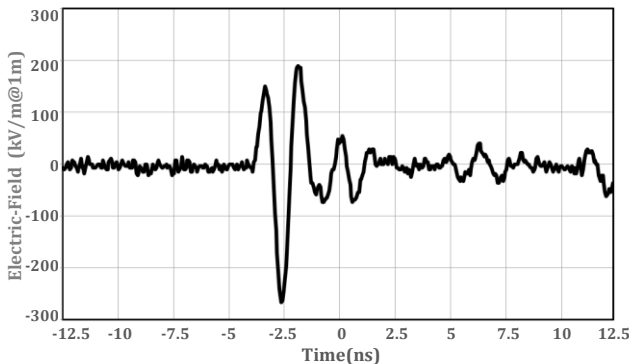
Electric-Field Waveform
